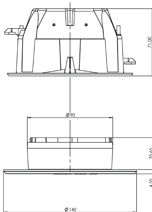
Figure 1: Soteria Dimension Optical Detector dimensional drawing
