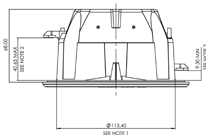
DETECTOR FITTED TO BACKBOX
